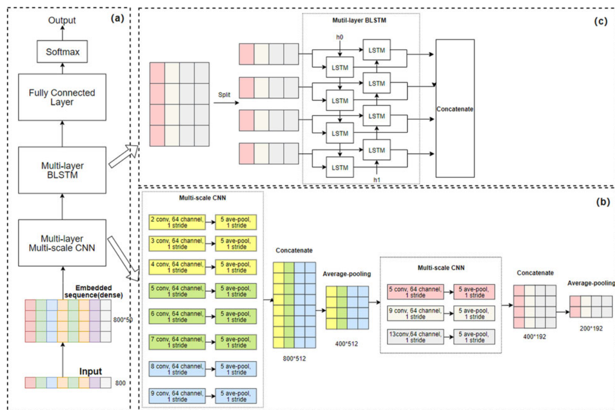
Fig. 1. The architecture of CLPred. (a) The overall workflow of CLPred. (b) The architecture of the CNN module. (c) BLSTM module. The discrete raw sequence is transformed into a dense, continuous vector through feature embedding and then fed into the CNN layer with multi-scale convolution kernels to capture local amino acid k -mers features. The extracted characteristic map of the CNN layer is passed to BLSTM concatenating the forward and backward information to capture the long-range interaction characteristics between k -mers. Finally, all the BLSTM outputs are passed to the fully connected layers to produce protein crystal prediction scores
