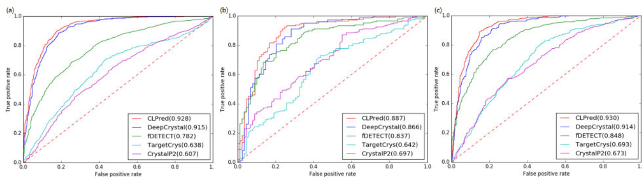
Fig. 2. ROC curves for the five predictors of the three different test sets. (a) ROC curve for DC_final, (b) ROC curve for SP_final dataset and (c) ROC curve for TR_final dataset. The AUC values of the five predictors are shown in the figure legend
