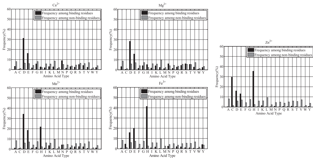
Fig. 1. Frequencies of the 20 native amino acids among binding and nonbinding residues for Ca 2+ , Mg 2+ , Mn 2+ , Fe 3+ , and Zn 2+ .
