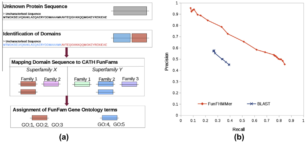
Fig. 4. (a) Protocol for function prediction using the CATH FunFams. The multi-domain architecture (MDA) of the query protein sequence (shown as a grey box) is first identified. Two domains are identified in the query sequence (shown as blue and red boxes), which are then mapped to their closest CATH FunFam match. The GO annotations of the closest FunFam are then transferred to each of the domain regions, which together make up the GO annotations for the query sequence. (b) Precision-Recall graph showing the performance of FunFHMMer (in red) compared to BLAST (in blue).
