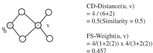
Fig. 6. CD-Distance and FS-Weight computation.
